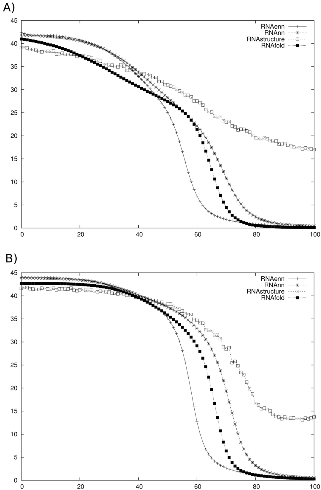
Figure 5. Melting curves for two small nucleolar RNAs (snoRNA) from family RF00158 from Rfam version 9.0 [56]. For each RNA sequence, over a range of temperatures, temperature-dependent base pair probabilities were computed using four different software packages: RNAenn, RNAnn, version 1.8.5 of RNAfold [40] and RNAstructure [38]. The software RNAenn (RNA extended nearest-neighbor) is our implementation of the algorithms described in this paper, while the software RNAnn (RNA nearest-neighbor) is our implementation of the following algorithms: Zuker's minimum free energy structure algorithm [51], McCaskill's partition function algorithm [19], and the Ding-Lawrence sampling algorithm [22].
