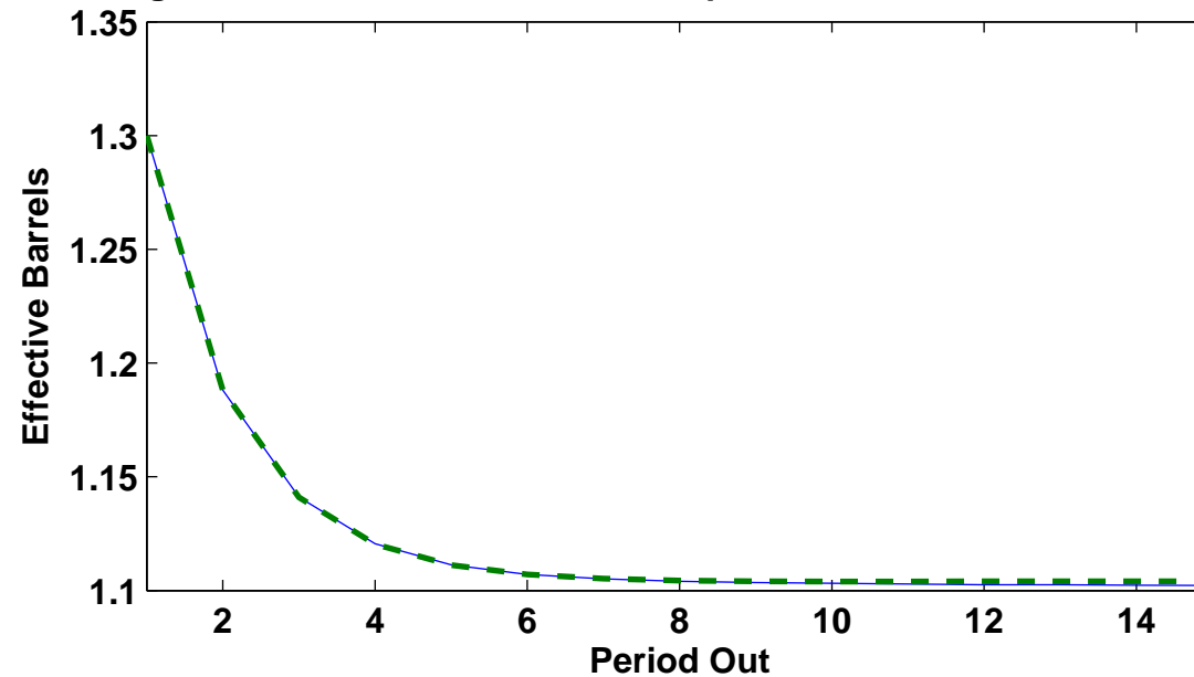
Figure 7d: Effective Production Response to Positive Growth Shock
