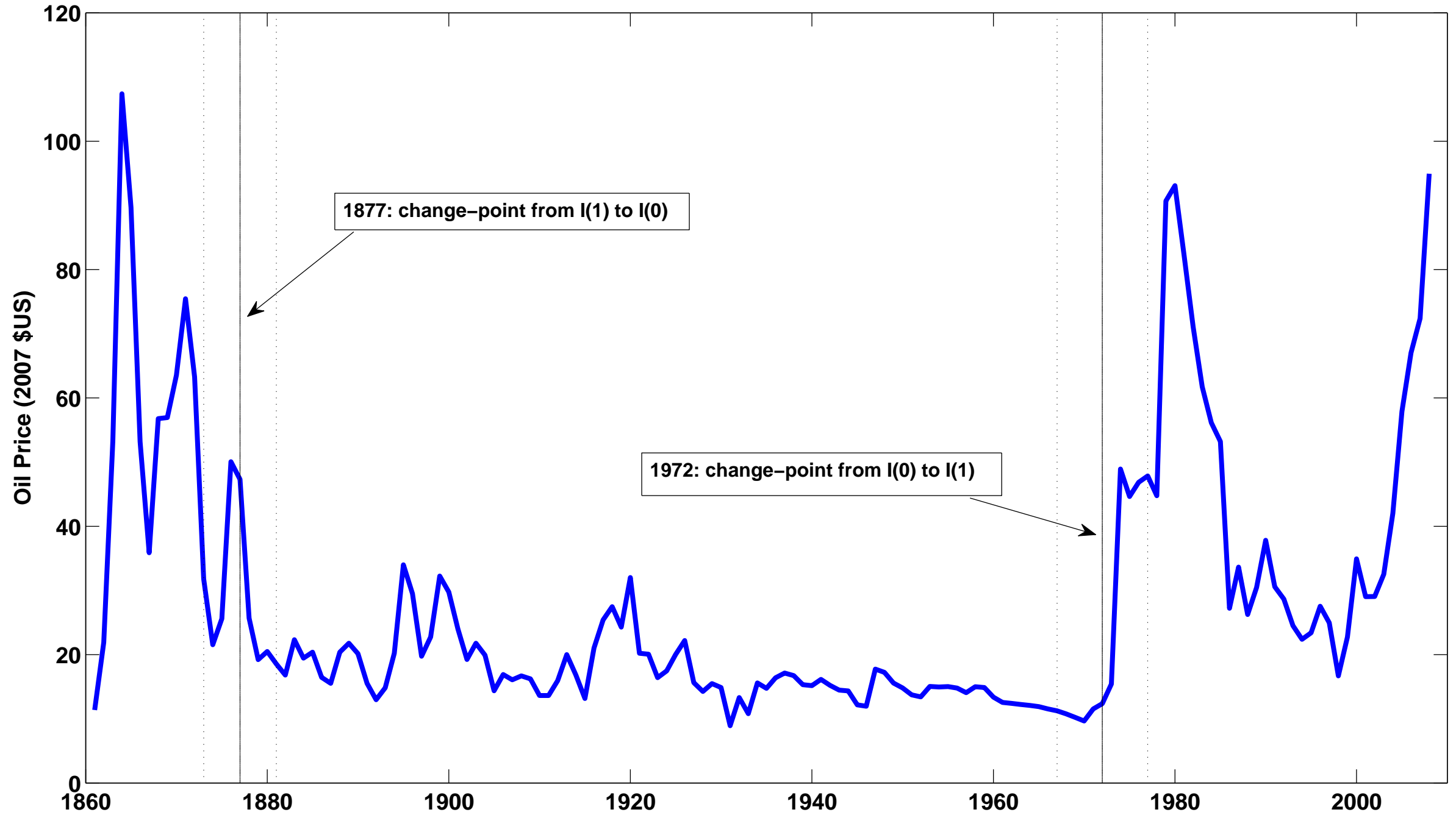
Figure 1: The Real Price of Oil 1861–2008
